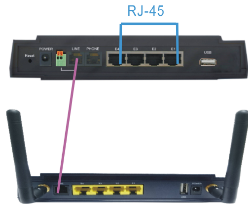
Figure 2.1 VC-400RTWU line ports straight connection
